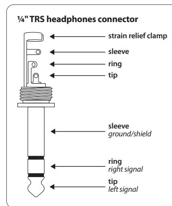
Fig. 4.5: 1/4" TRS connector for headphones
