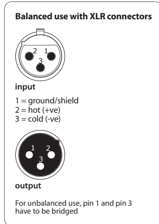
Fig. 4.2: XLR connections
