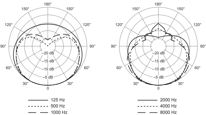
Polar Pattern
