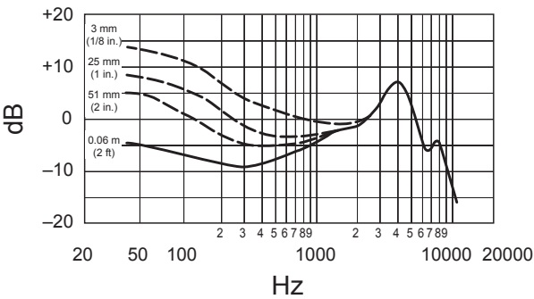
Frequency Response
