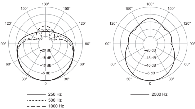
Polar Pattern
