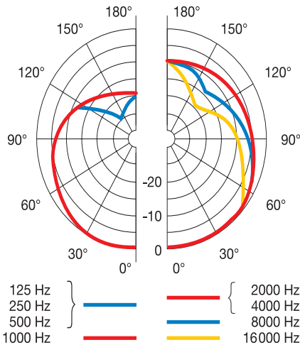
Polar Diagram C214
