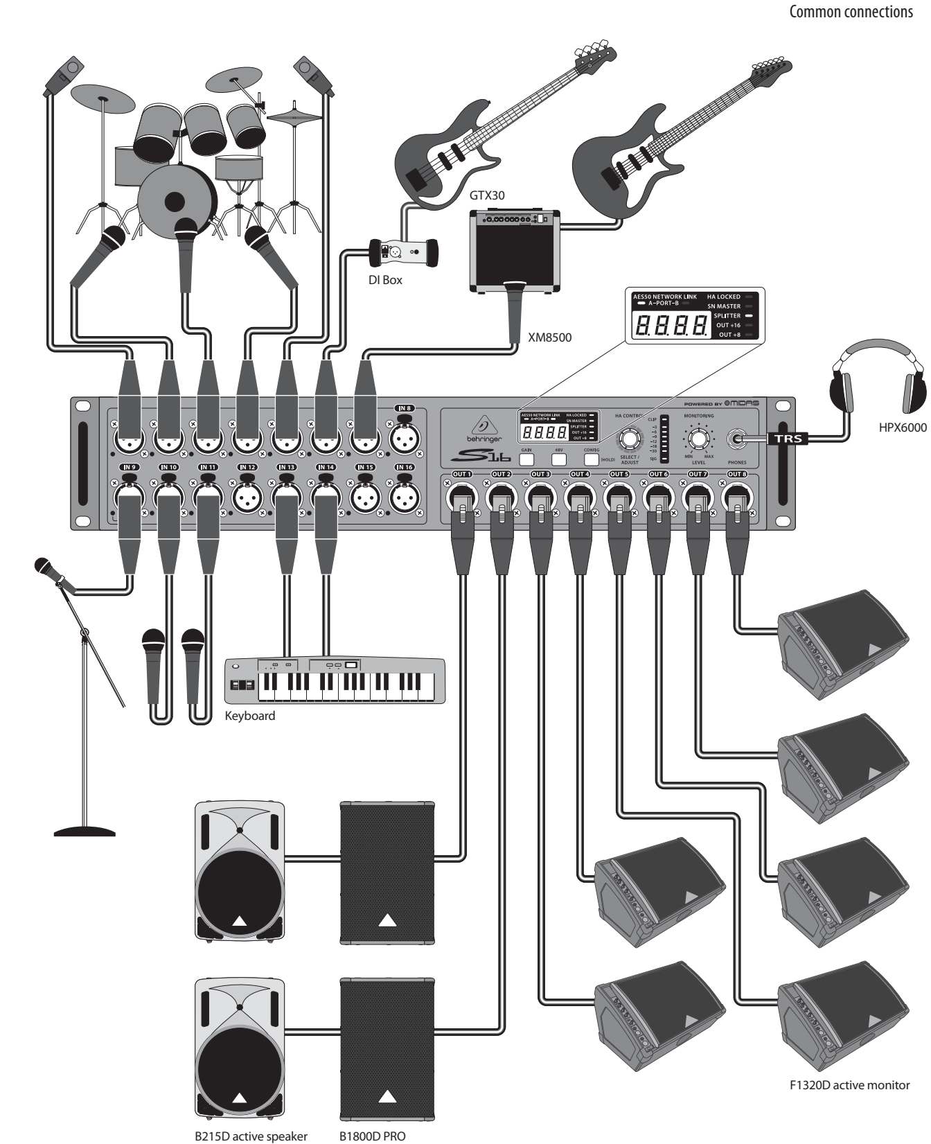
Common connections
